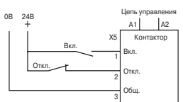
AF400 ... AF750-30-11, AF400 ... AF750-30-22
