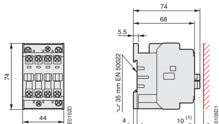
A 9, A 16, N
